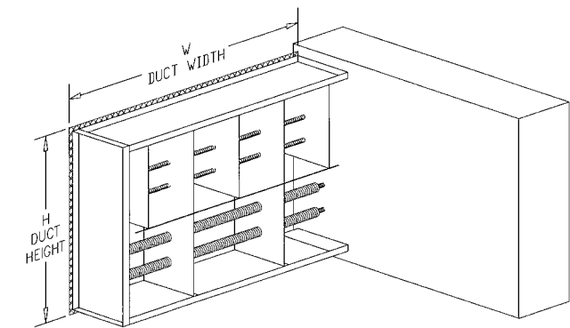
Figure 69. Slip-in Duct Heater
