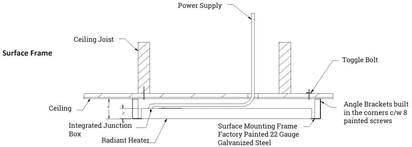
Cutaway View of AS Series
